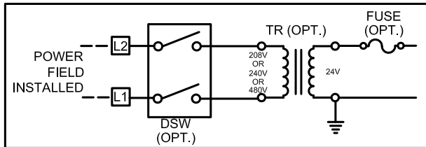
OPTIONAL TRANSFORMER / VOLTAGES
