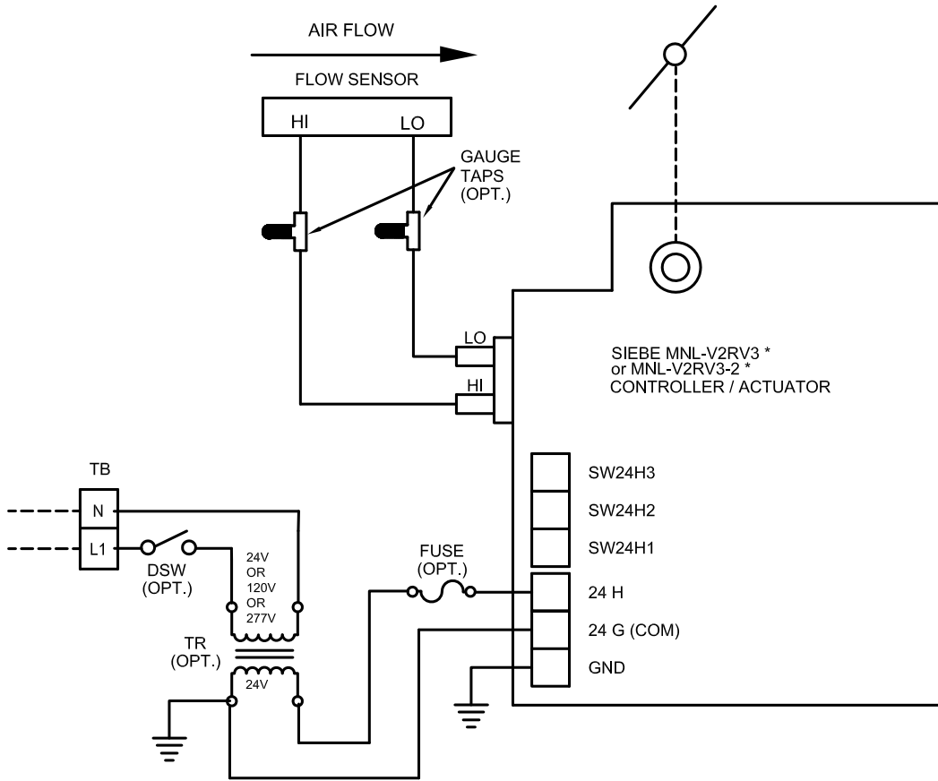
OPTIONAL TRANSFORMER / VOLTAGES
