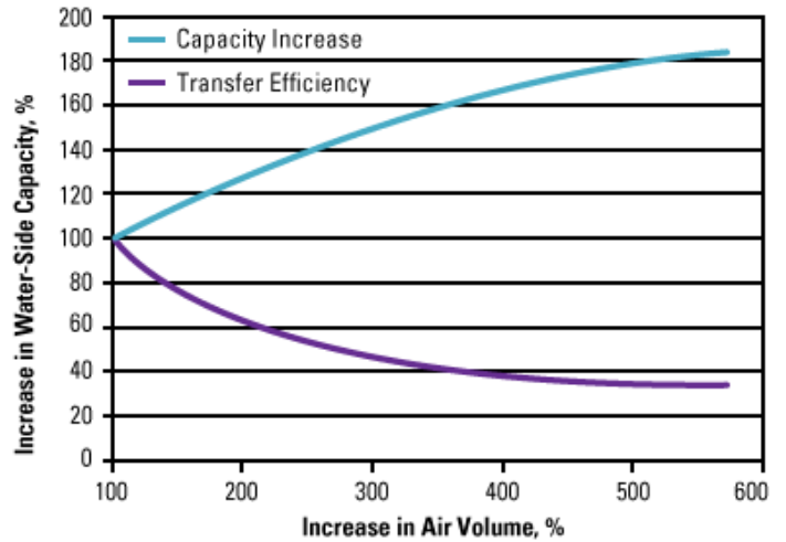
Figure 3: Capacity vs. air volume.
