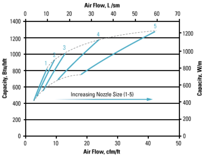
Figure 2: Capacity of a typical active beam v. primary air flow according to nozzle size.
