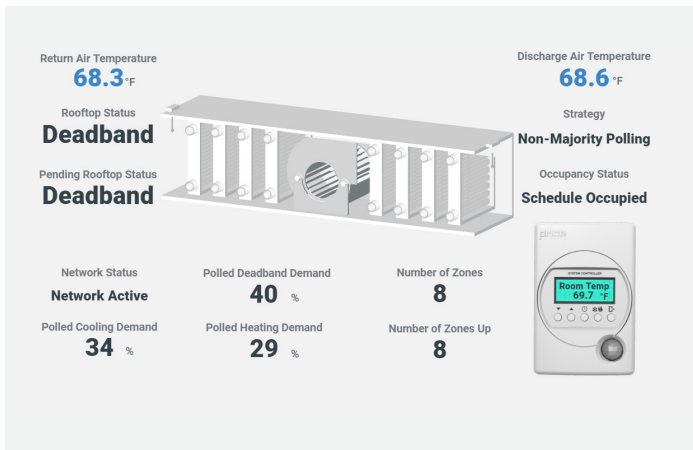
Price Rooftop Unit Controller (PRTU) Graphic
