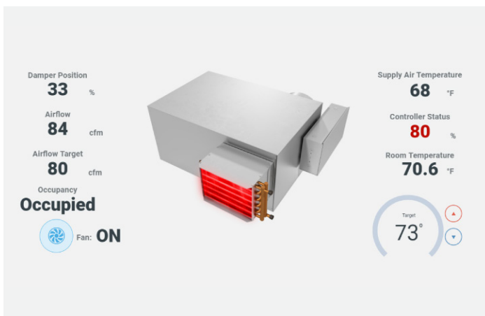
Price Intelligent Controller (PIC) Graphic
