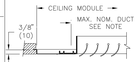
SPLINE CEILINGS: 4P 4PA
