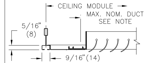
FINELINE LAY-IN PANELS: 17P 17PA
